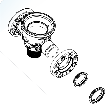
Connection Type: Victaulic/Threaded/Optionally 3" Flanged
