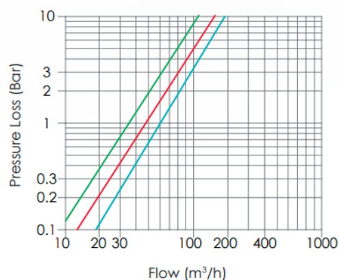
HEAD LOSS
